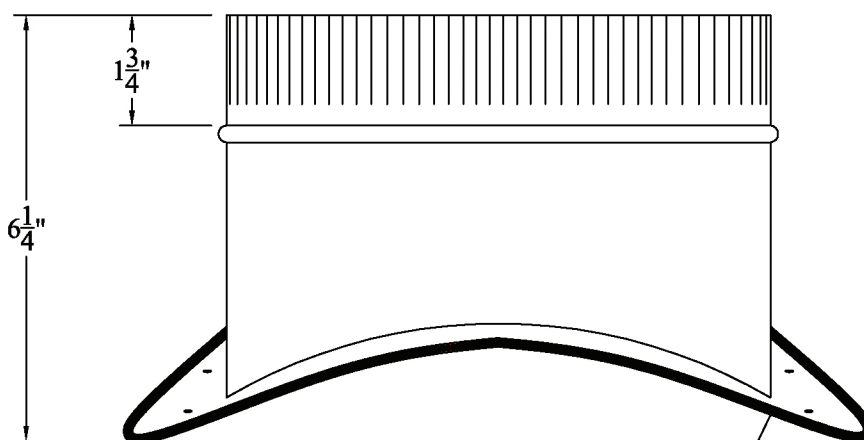
Metal Flange with Air Tite Gasket
