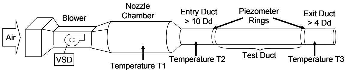
Figure 1: Test Setup
